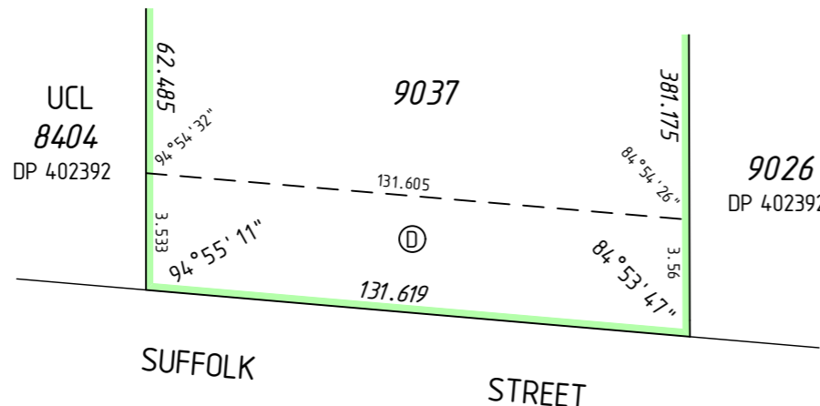
ENLARGEMENT "A1" NOT TO SCALE
